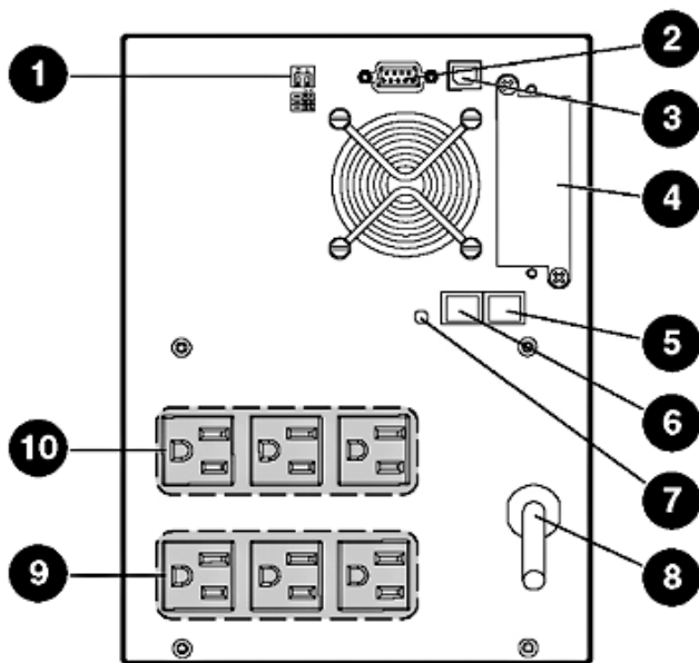
Rear Panel
