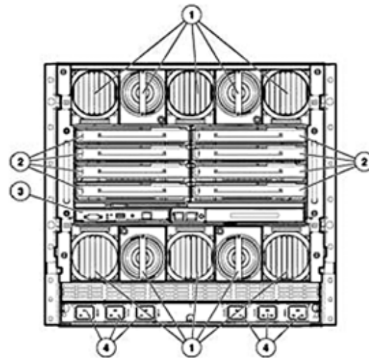
HPE BladeSystem c7000 Enclosure - Rear View
