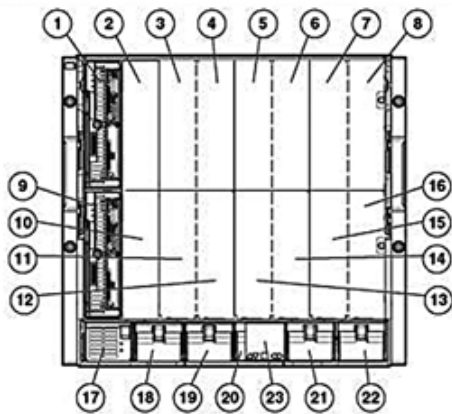
HPE BladeSystem c7000 Enclosure - Front View
