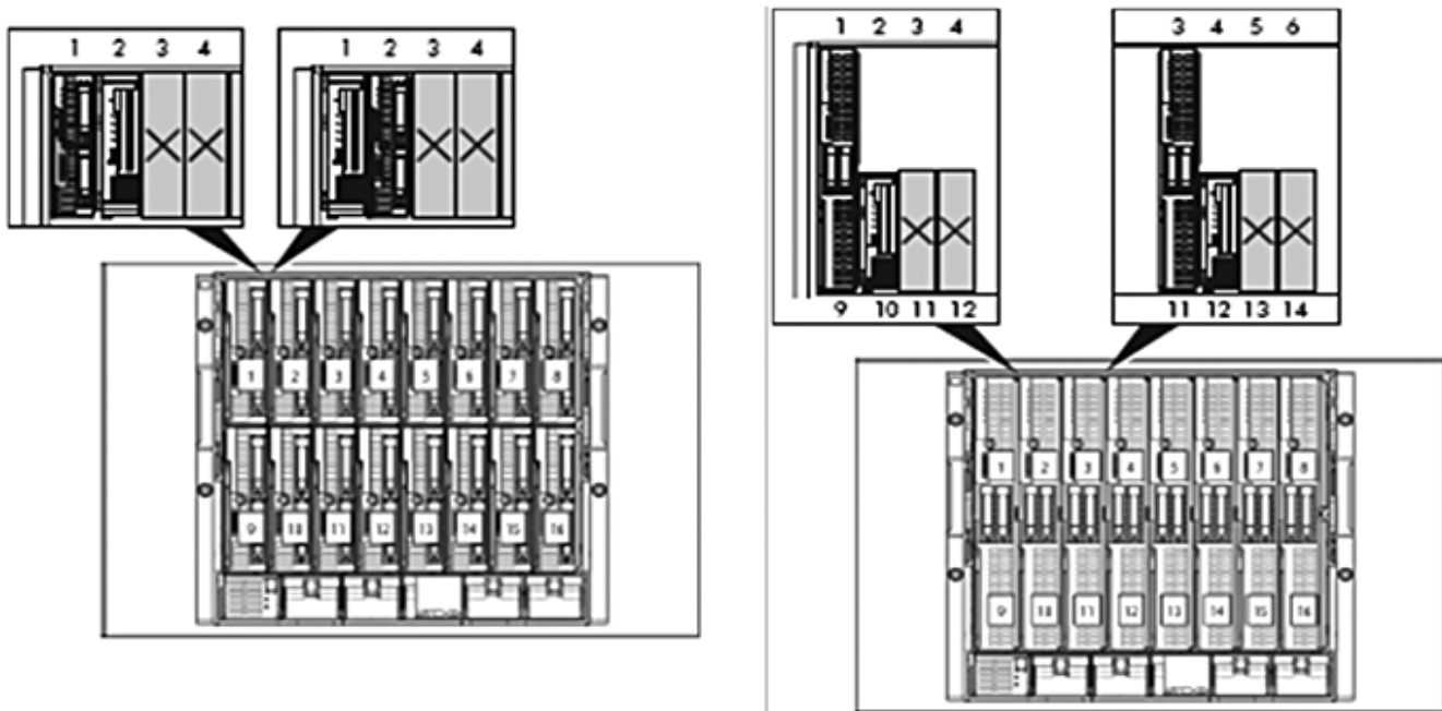
Figure 1 Installing an expansion blade adjacent to a half-height server blade. Figure 2 Installing a single expansion blade adjacent to a full-height, single-wide server blade.
