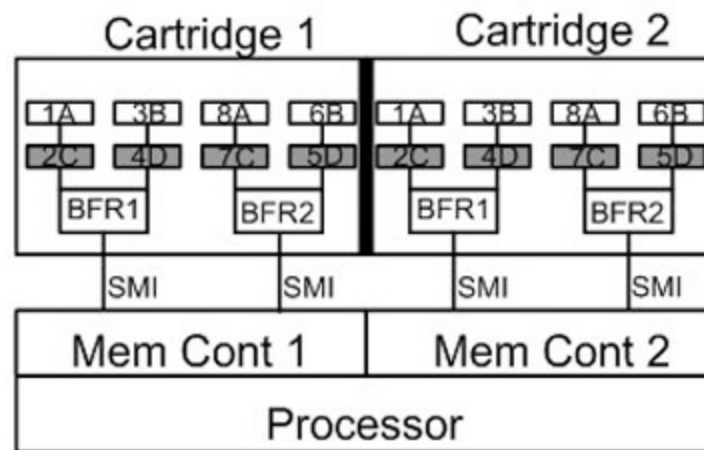
Figure 1 Processor/Memory interconnect
