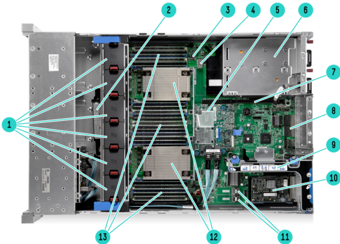
Internal View
