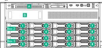
40 SFF hot-plug drives with 6 SFF NVMe SSD
