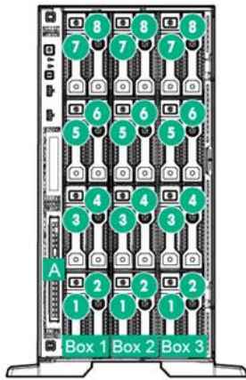
24 LFF hot-plug drive model (Rack)
