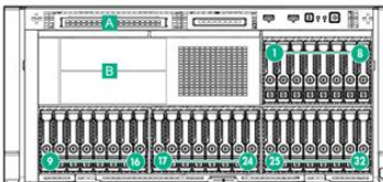
16 LFF hot-plug drives with LFF media cage
