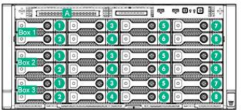
32 SFF hot-plug drives with SFF media cage
