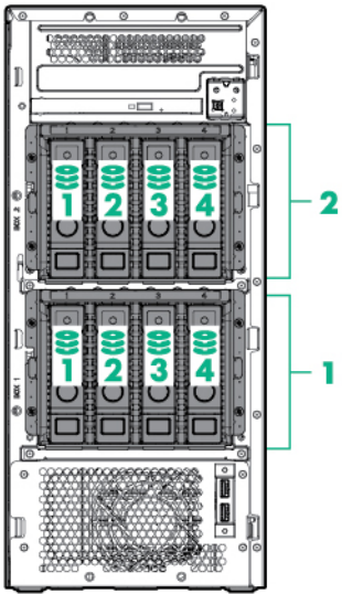
8-bay SFF hot-plug drive model
