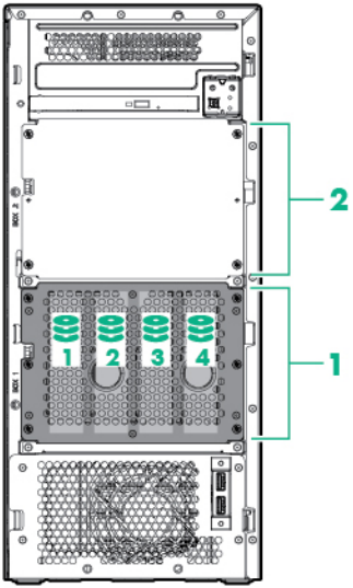
4-bay LFF hot-plug drive model
