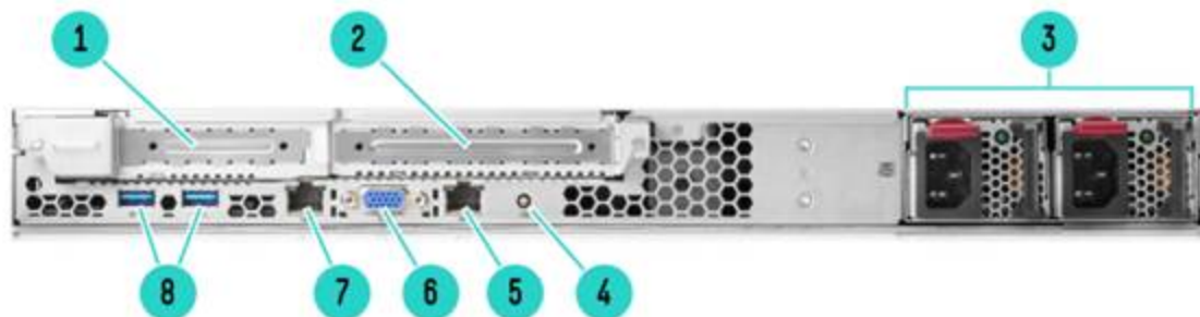
Rear View
