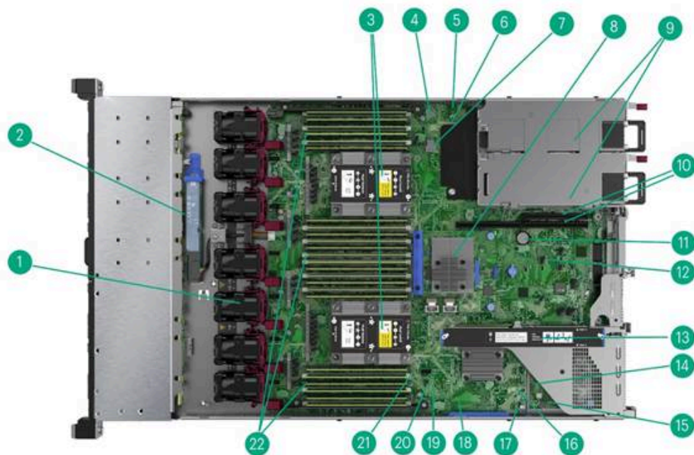
Internal View - Standard for all DL360 Gen10
