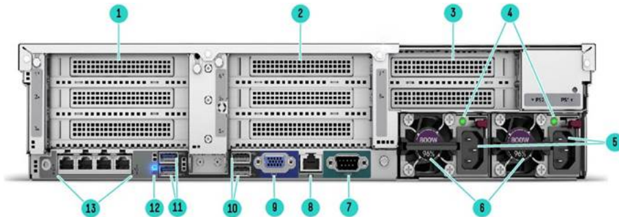
Rear View - DL560 Gen10
