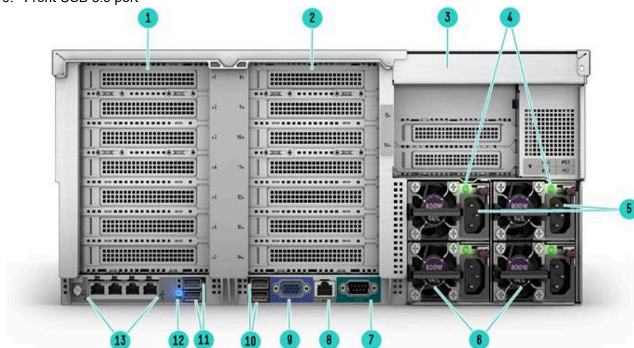
HPE ProLiant DL580 Gen10 Server Rear View
