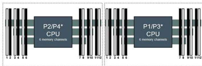
HPE DL360/DL380/DL560*/DL580* Gen10 Servers (2 slots per channel)
