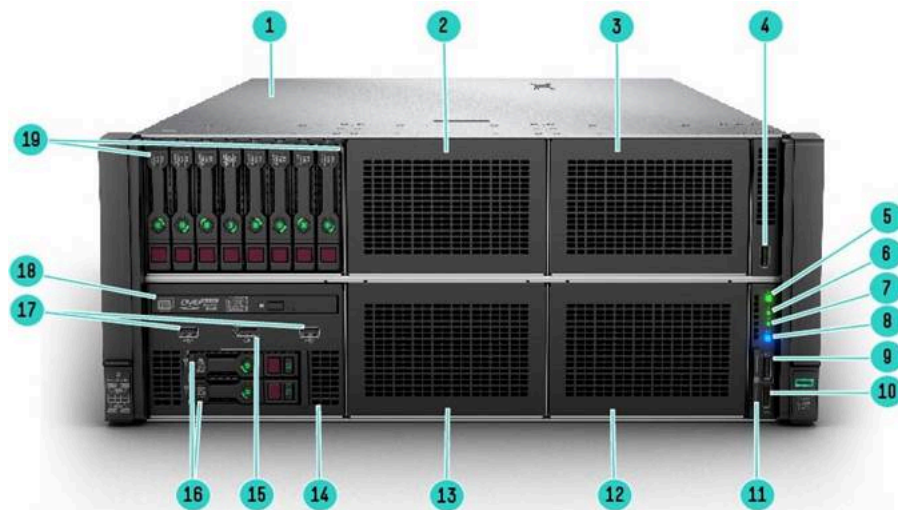
HPE ProLiant DL580 Gen10 Server Front View
