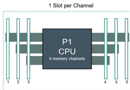
HPE ML110 Gen10 Server (Front of Server)
