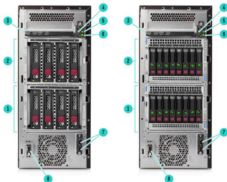
Front View (details for 8LFF and 16SFF)
