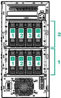
4-bay LFF hot-plug drive model
