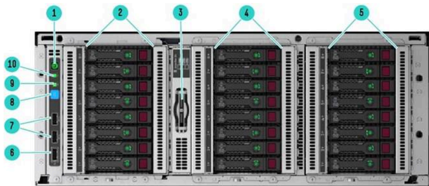
Front View - SFF chassis with optional Gen10 8SFF HDD Cage Kits shown (Rack mode)
