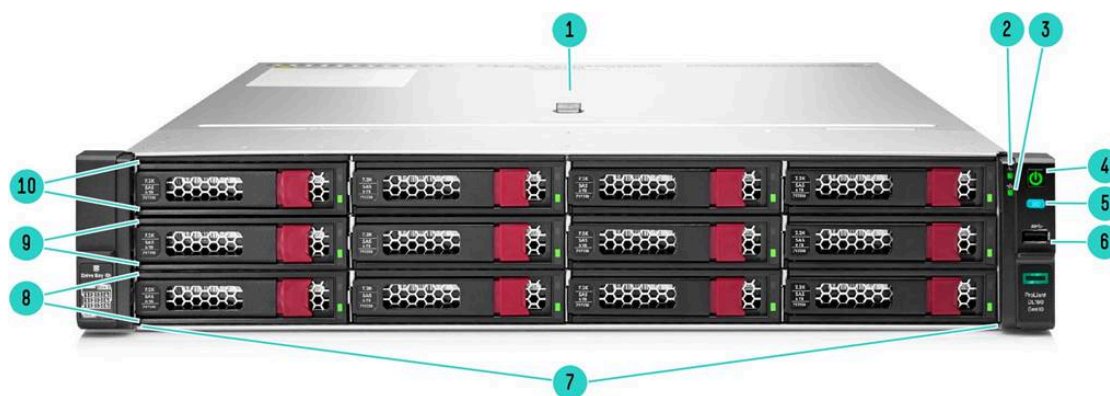
12LFF Chassis - Front View
