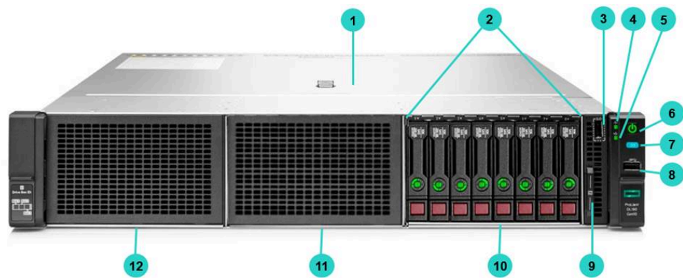
8SFF Chassis - Front View
