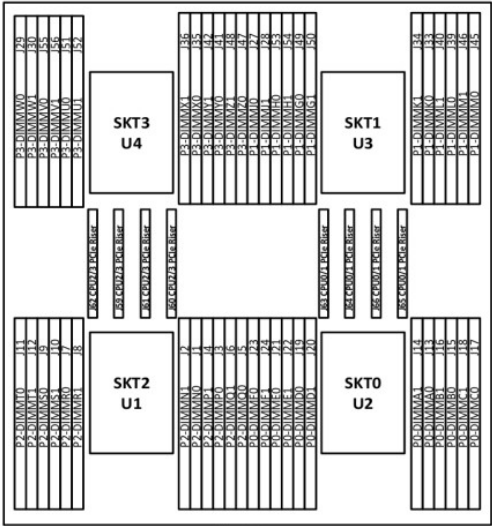
Superdome Flex DIMM Arrangement
