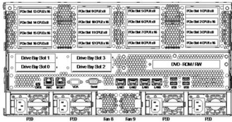
Base Chassis rear view (16-slot) 16x LP PCIe IO slots 4x HDD/SSD bays 1x DVD-R/DVD-RW bay 4x Ethernet ports 4x Power supplies 2x Superdome Flex ASIC fans
