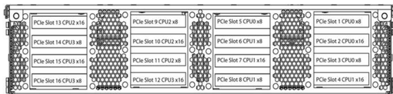
16-slot configuration
