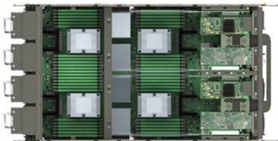
Chassis top view
