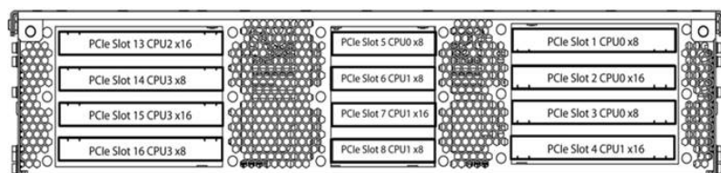
12-slot configuration
