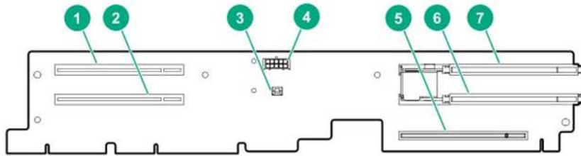
Right 4xGPU Riser Kit (P19233-B21)
