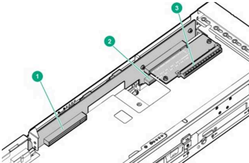
2U P2 Secondary Riser Cage Assembly (874851-B21)
