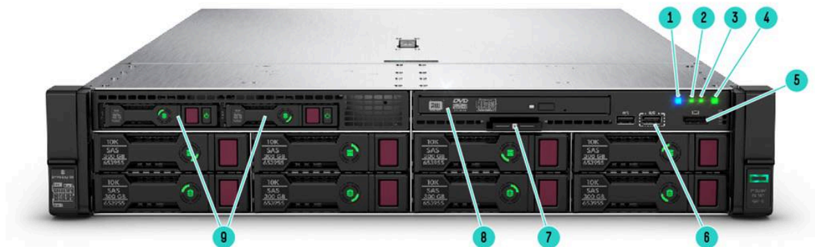
HPE ProLiant DL385 Gen10 Server - Front View
