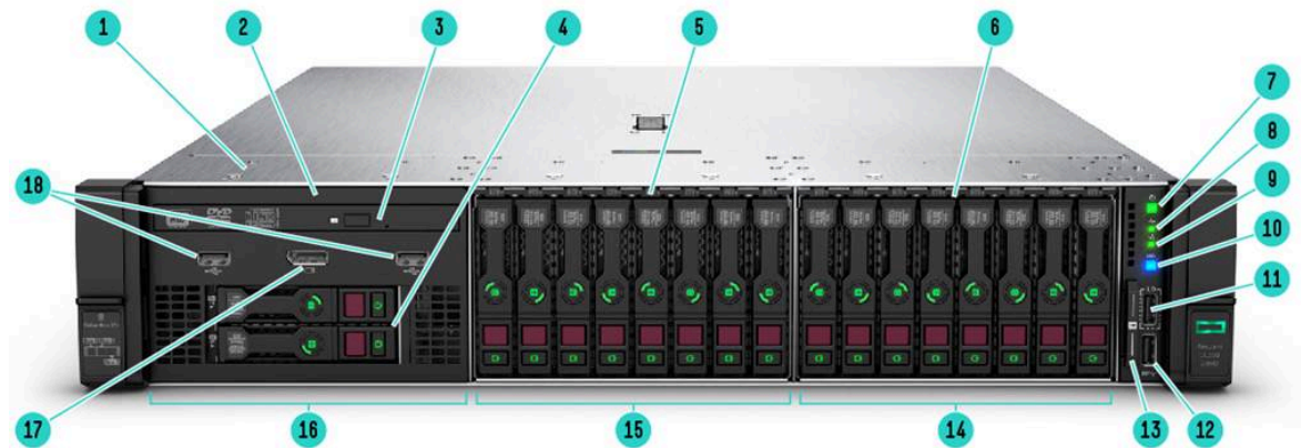
HPE ProLiant DL385 Gen10 Server - Front View
