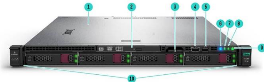
4LFF Front View - with Optional ODD shown
