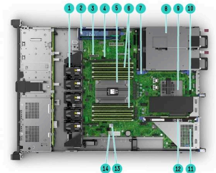
Internal View 8SFF chassis -with optional FlexLOM, Smart array shown
