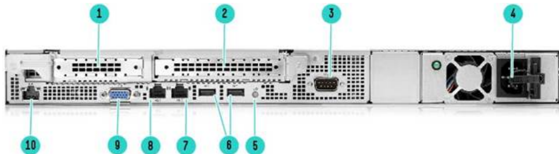
Rear View - Standard for all DL20 Gen10
