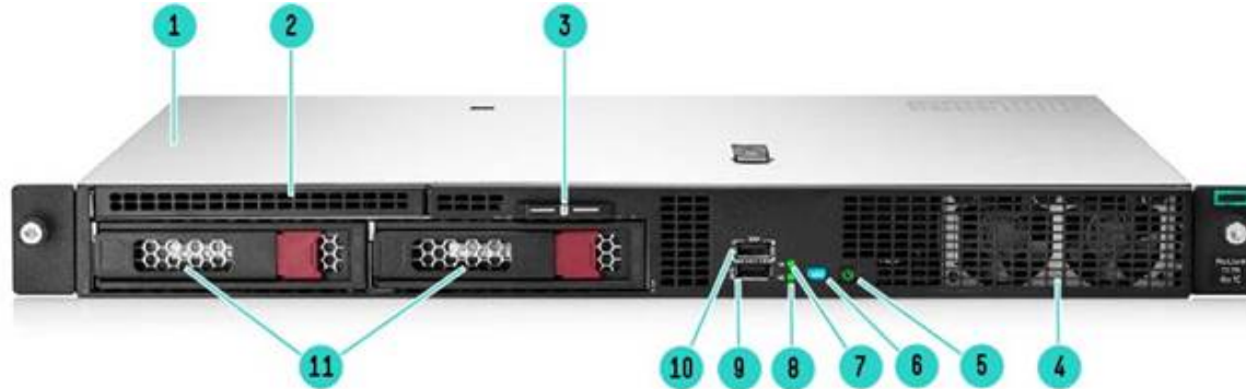
2 LFF Front View
