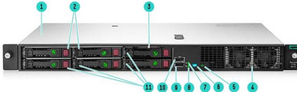
4 (+2) SFF Front View
