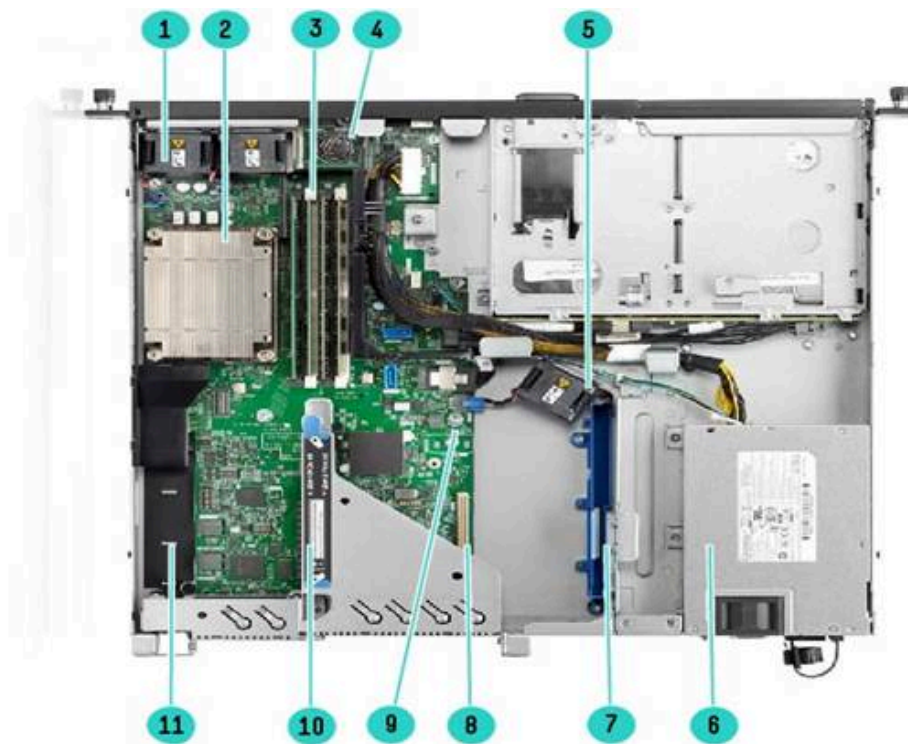
Internal View - Standard for all DL20 Gen10
