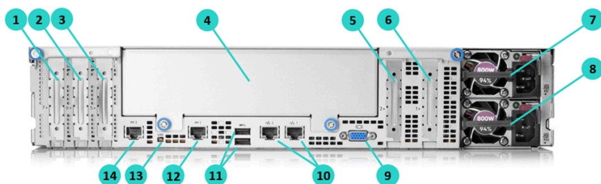
Standard for all Apollo 4200 Gen10 - Rear View
