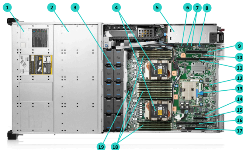
Standard for all Apollo 4200 Gen10 - Internal View
