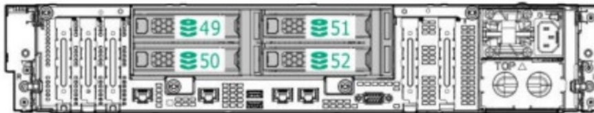
4LFF hot-plug rear drive numbering
