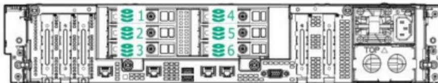
6SFF NVMe rear drive numbering
