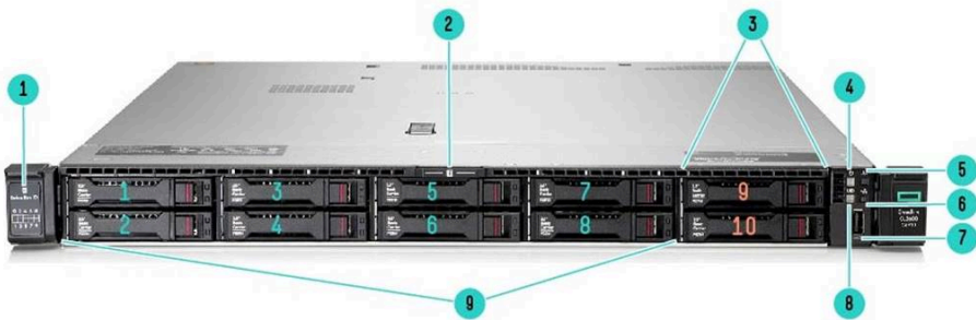
Premium 10SFF NVMe Front View
