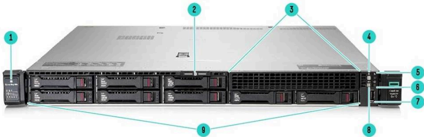
8SFF Front View- Standard 8SFF shown
