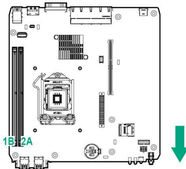
Maximum Memory
