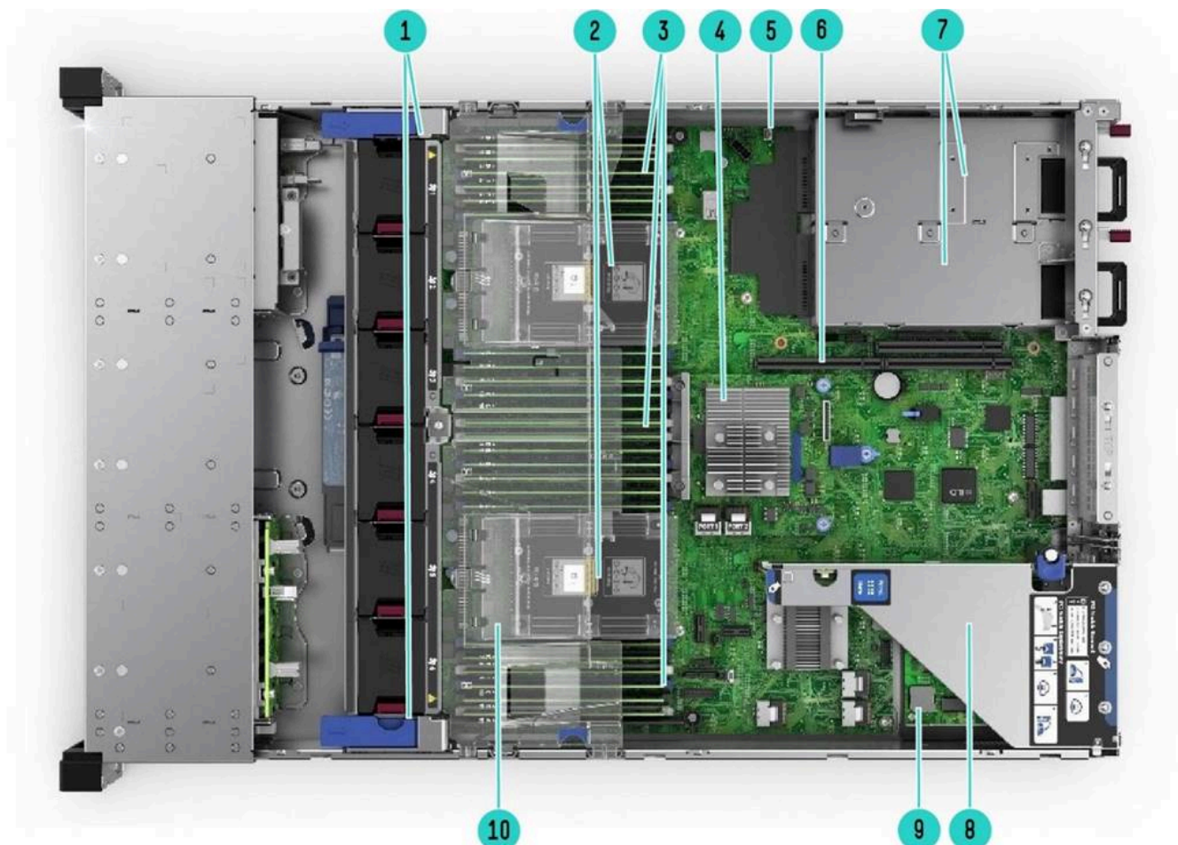
Internal View - with 2 nd CPU and FlexLOM shown
