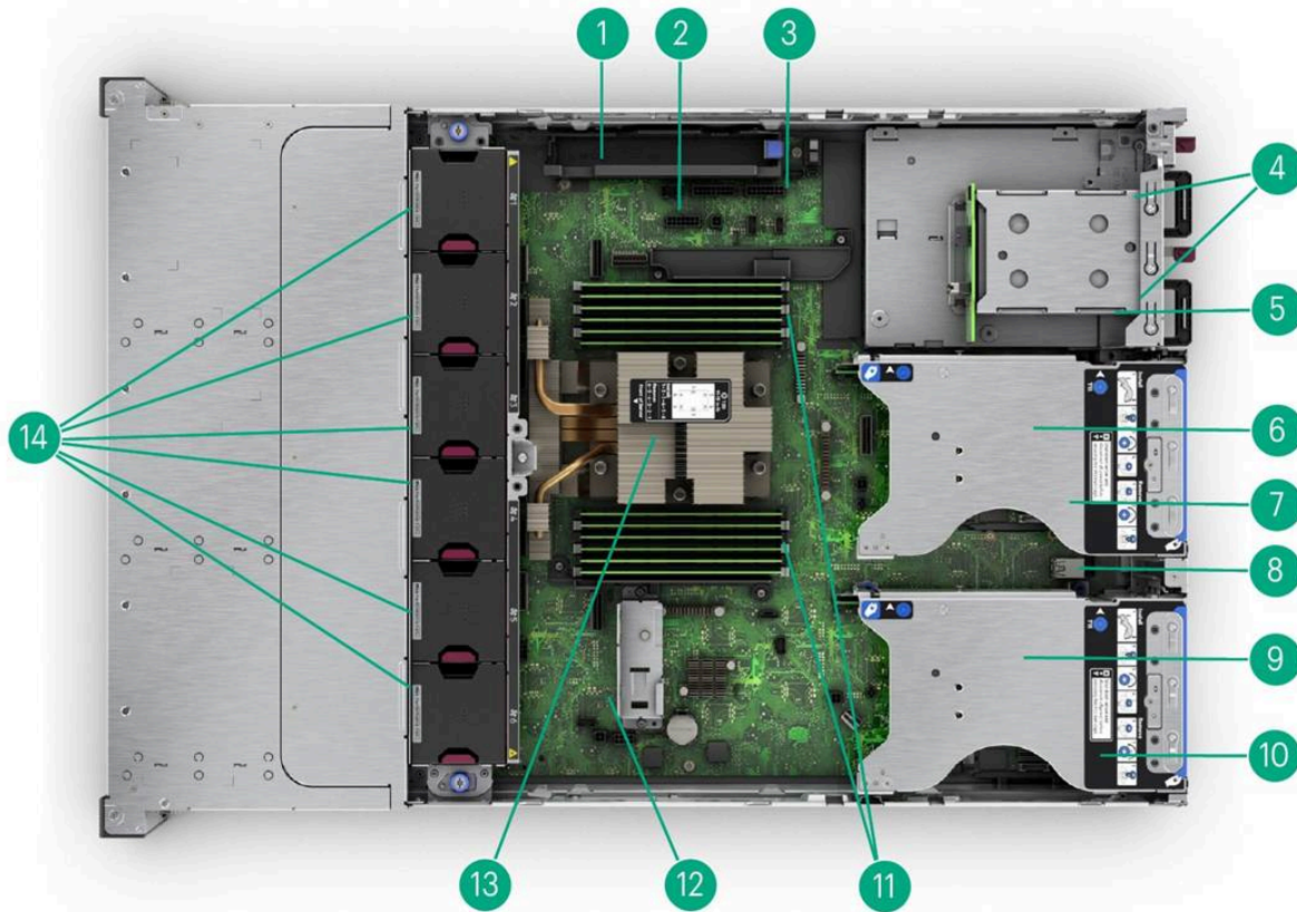
Internal View - 2SFF rear cage shown
