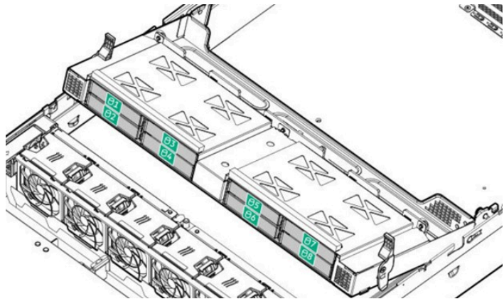
8 SFF Mid Tray
