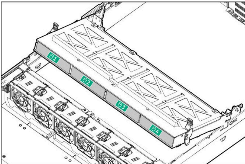
Midplane Box (LFF)
