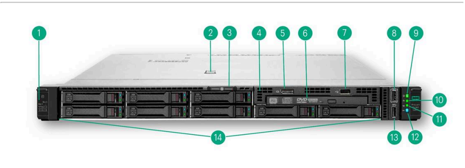
8 SFF Front View- 8 SFF + optional Universal Media Bay, optical drive, DisplayPort, USB2.0 and SAS drives shown
