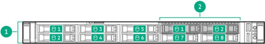
8 SFF + 2 SFF (optional) device bay numbering
