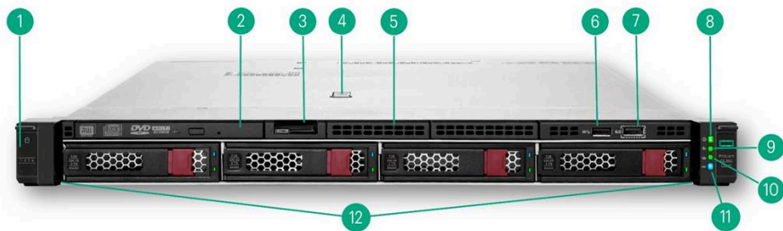
4 LFF Front View - 4 LFF + optional Optical drive, DisplayPort, USB2.0 and SAS drives shown
