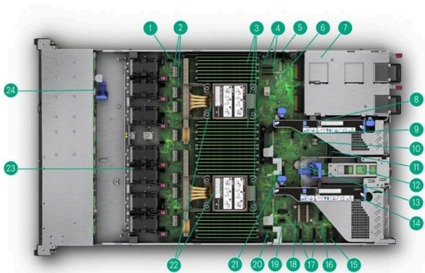
Internal View - Standard for all DL360 Gen11
