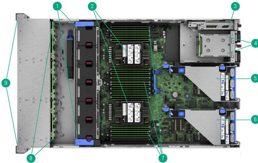
Internal View 8SFF chassis
