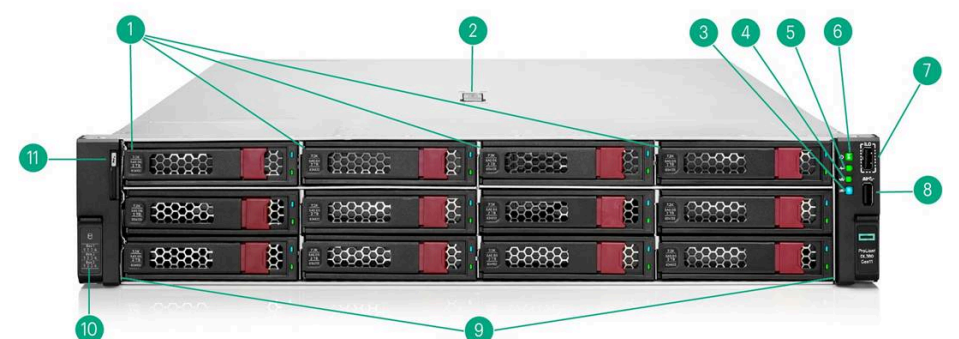
Front View - 12LFF chassis shown
