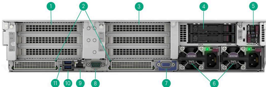
Rear View - Standard for all DL380 Gen11
