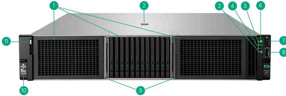
Front View -12EDSFF chassis shown
