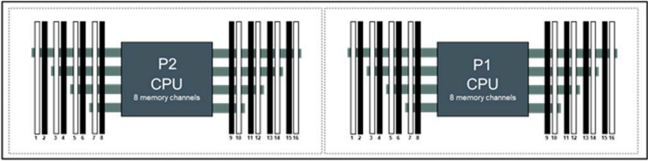
HPE ML350 Gen11 Server (Front of server)
