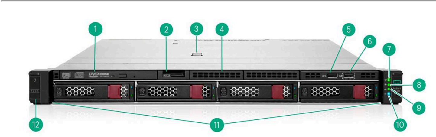
4 LFF Front View - 4 LFF + optional Optical Drive and SAS drives shown
