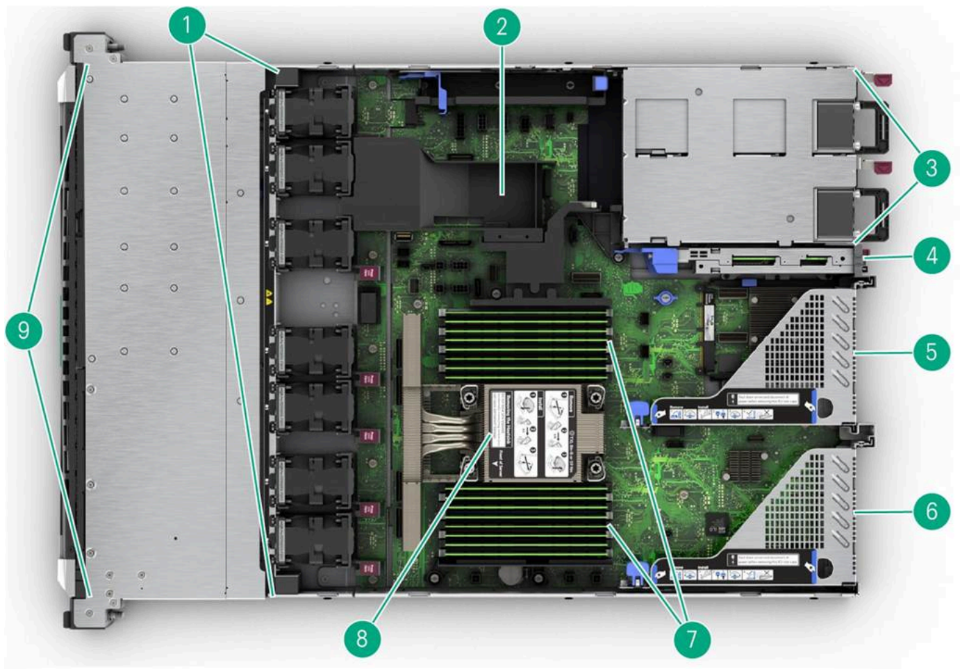
Internal View - Standard for all DL320 Gen11
