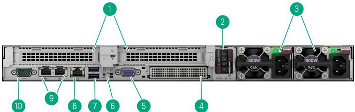
Rear View - Standard for all DL320 Gen11
