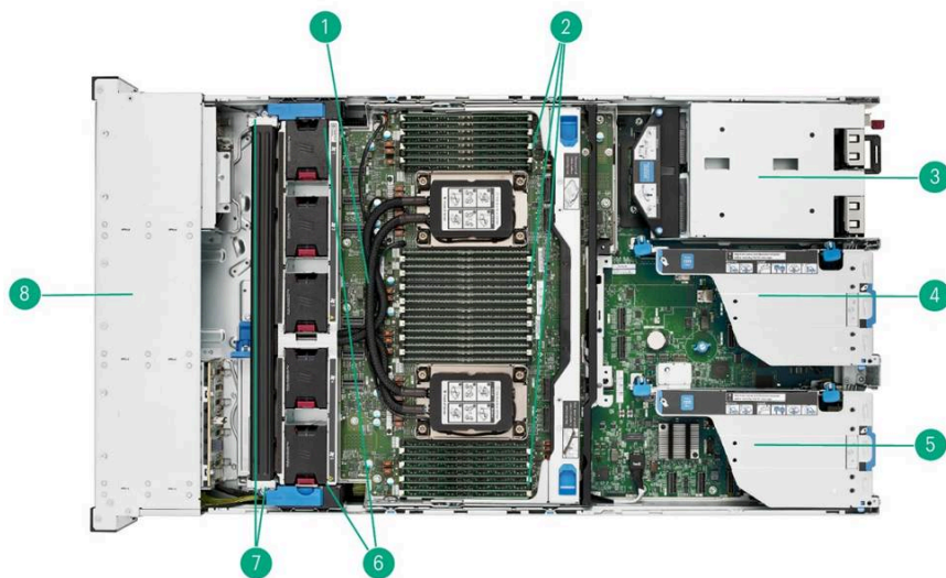
Internal View Liquid Cooling Chassis
