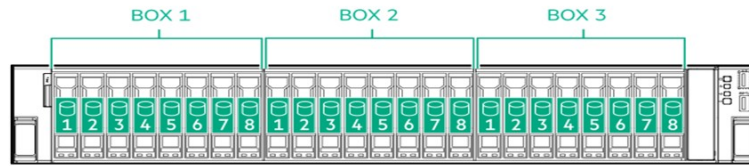
DL560 Gen11 24SFF Front View
