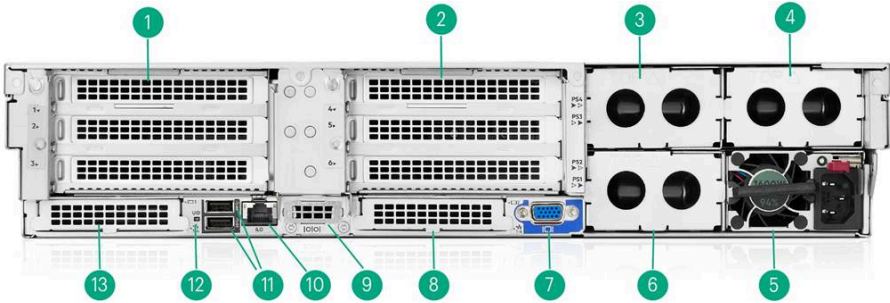
Rear View - Standard for all DL560 Gen11
