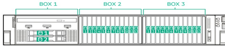
DL560 Gen11 12 EDSFF + Media Bay Front View
