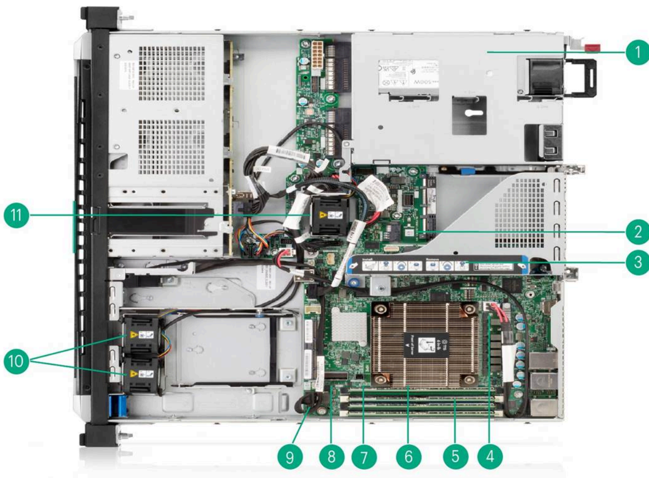
Internal View - Standard for all 4 SFF DL20 Gen11
