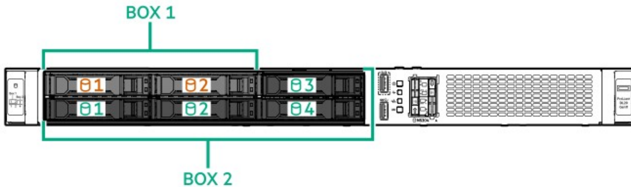
4 SFF + 2 SFF device bay numbering
