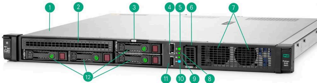
4 SFF Front View Gen11
