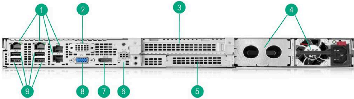
Rear View - Standard for all DL20 Gen11
